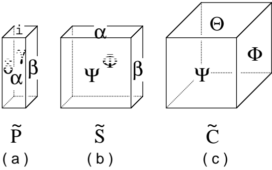
Fig. 7. The renormalized tensors (a) \tilde{P}_{\alpha\beta\gamma\delta}^i in eq.(4.4), (b) \tilde{S}_{\alpha\beta\gamma\delta}^{\Psi\Phi} in eq.(4.5), and (c) \tilde{C}^{\Psi\Phi\Theta} in eq.(4.2). The greek letters \alpha, \beta, \gamma, and \delta denote m -state renormalized in-line spins, and the capital ones \Psi, \Phi, and \Theta denote m' -state renormalized spin arrays.
