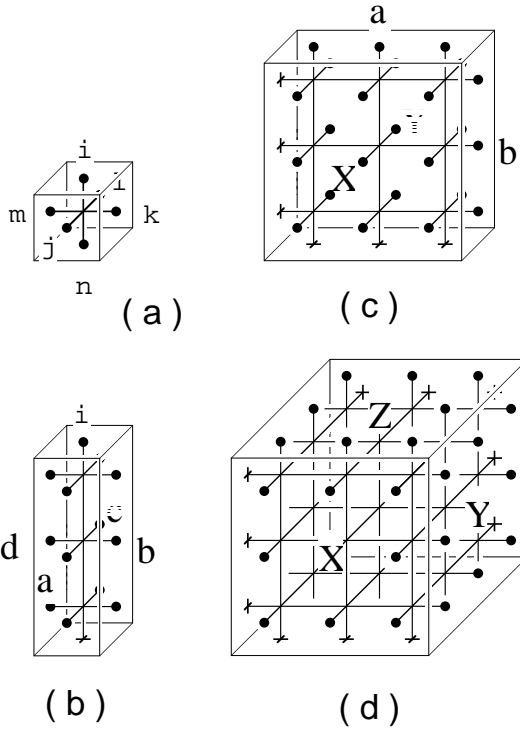
Fig. 4. Parts of the cubic cluster with linear dimension 2N : (a) Vertex weight W_{ijklmn} . (b) The tensor P_{abcd}^i . (c) The tensor S_{ab}^{XY} . (d) Corner Tensor C^{XYZ} . The cross marks \times represent the boundary spins.
